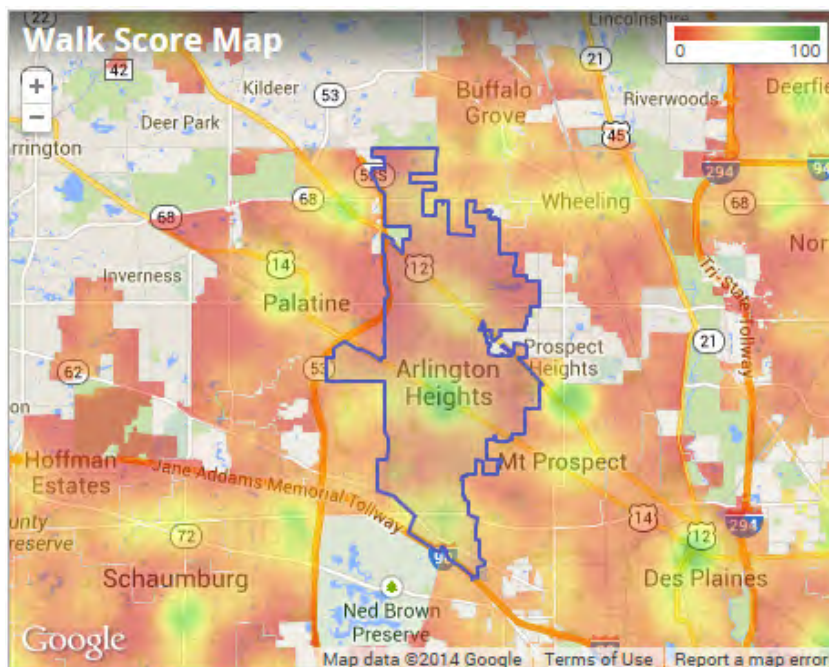
Figure 2.2 - Walkscore
