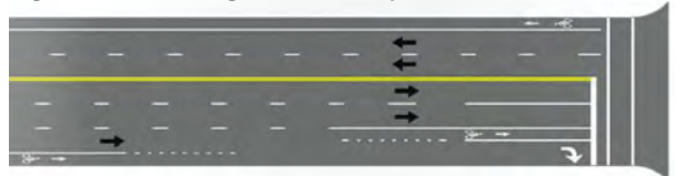
Figure 4.76 - Through Bike Lane Option D
